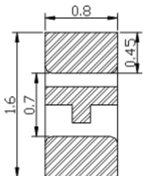
Package Outline Dimensions:
