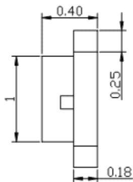
Paecommmended Soldering Pattern
