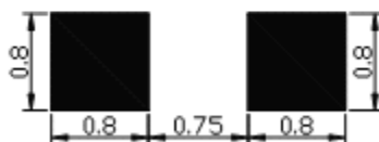
Paecommmended Soldering Pattern
